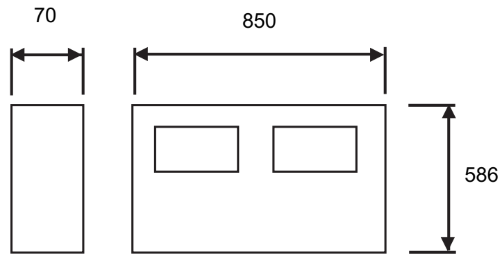
Score Box (HUB) (Dimensions in mm)
