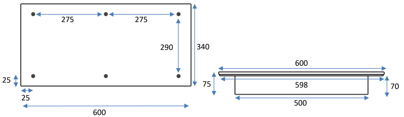
Figure 2: Target Mounting Points and Dimensions (Dimensions in mm)
